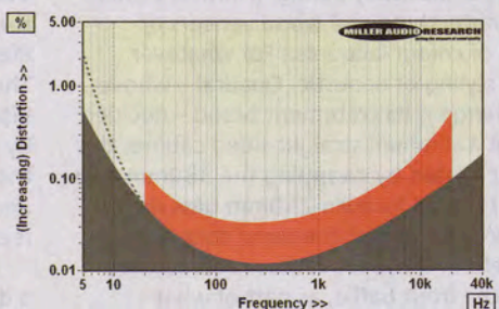
ABOVE: Distortion versus frequency, 5Hz-40kHz at 1W/8ohm (black) and 20Hz-20kHz at 10W (red)
