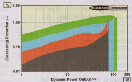
ABOVE: Dynamic power output versus distortion into 8ohm (black trace to 1%), 4ohm (red to 1%), 2ohm (blue to 2%) and 1ohm (green to 2%) speaker loads
